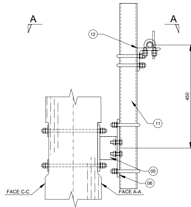
DETAIL H - Rx ANTENNA MOUNT Scale 1:10
