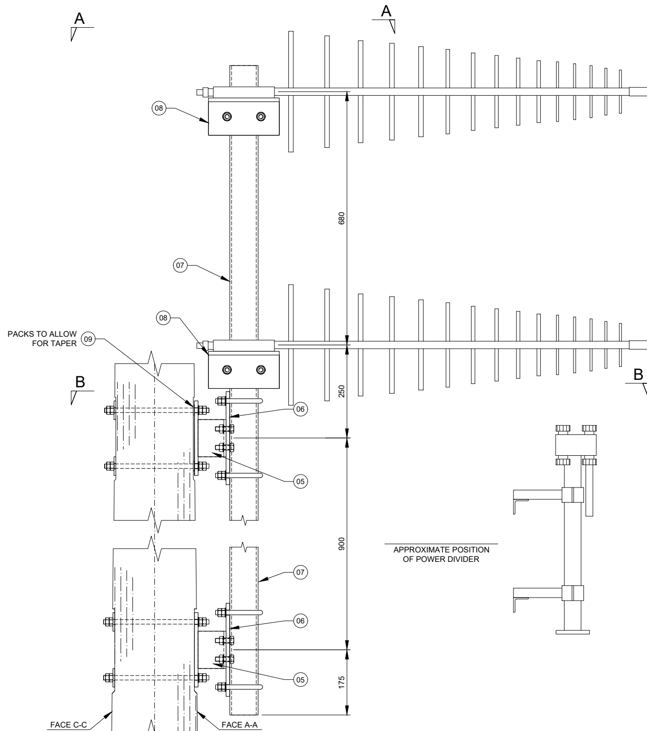
DETAIL G - Tx ANTENNA MOUNT Scale 1:10
